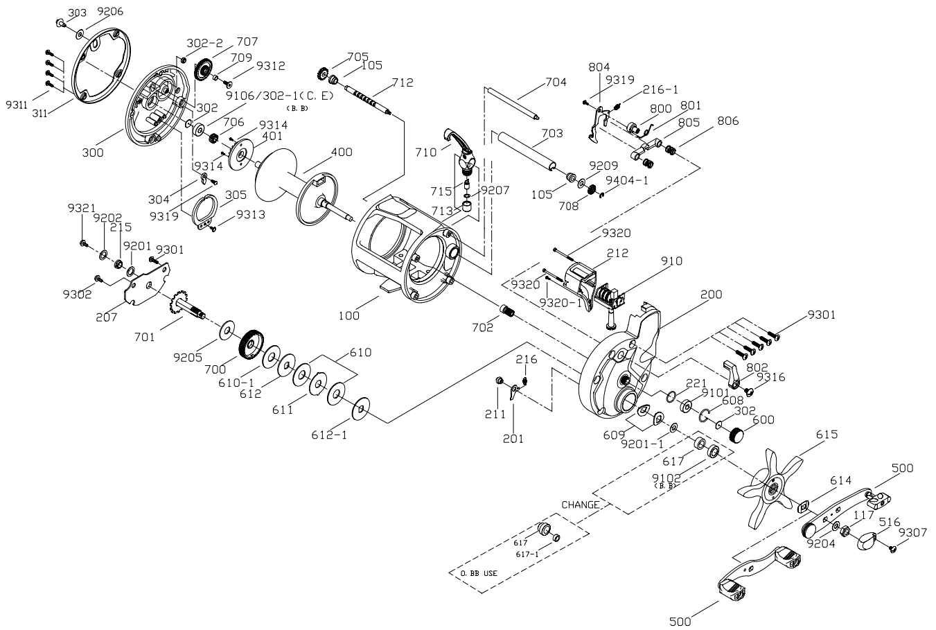
SD - 20D Spare Parts
